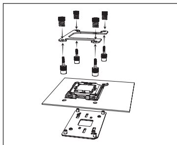
● AM4 / AM5
