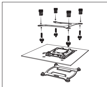
● Intel LGA 1700 / 1851
