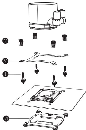
● Intel LGA 1700 / 1851
